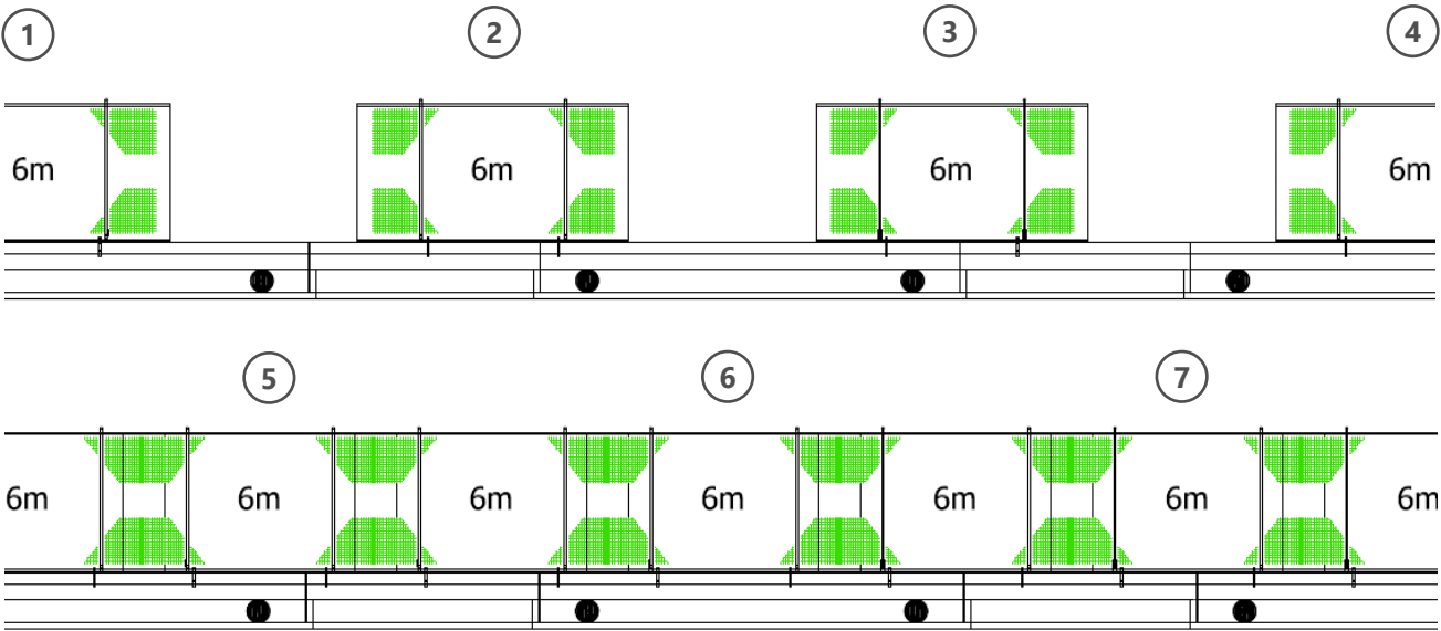
Example of an alternated catchfan installation with 7 pcs catchfan
