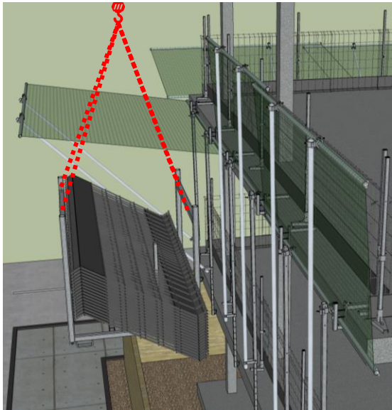
Fold the catchfan for lifting material close to the structure
