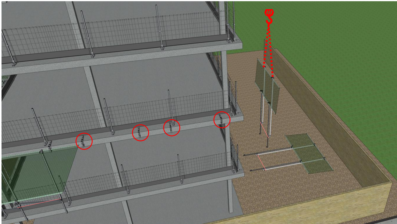
Pre-install the attachment
