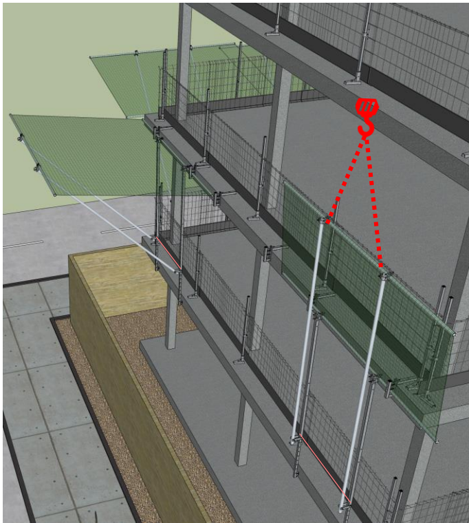
Insert catchfan into attachment & lock it
